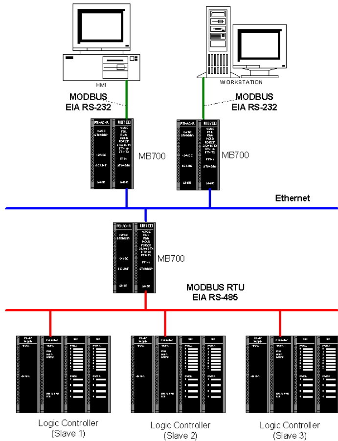
Fig. 5.14 – MB-700 working as Bypass Serial To TCP
