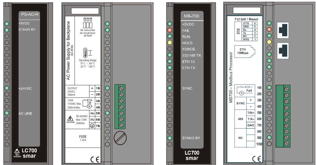
PS-AC-R (Power Supply) and MB-700
