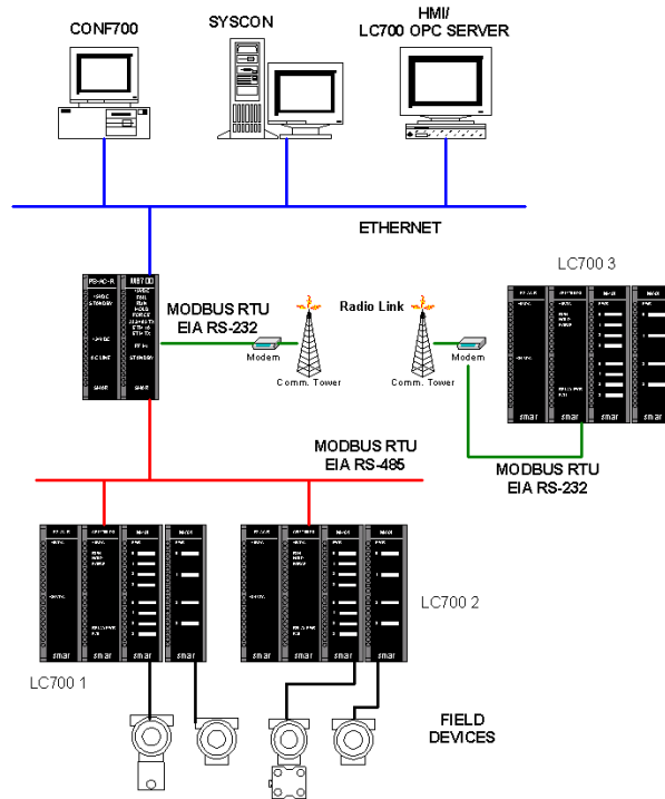
Fig. 5.1 – MB-700 as a serial MODBUS master
