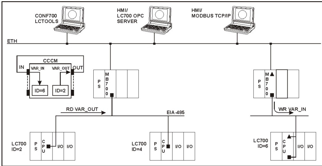
Fig. 5.3 – MB-700 working as Peer-To-Peer in the Serial and TCP/IP
