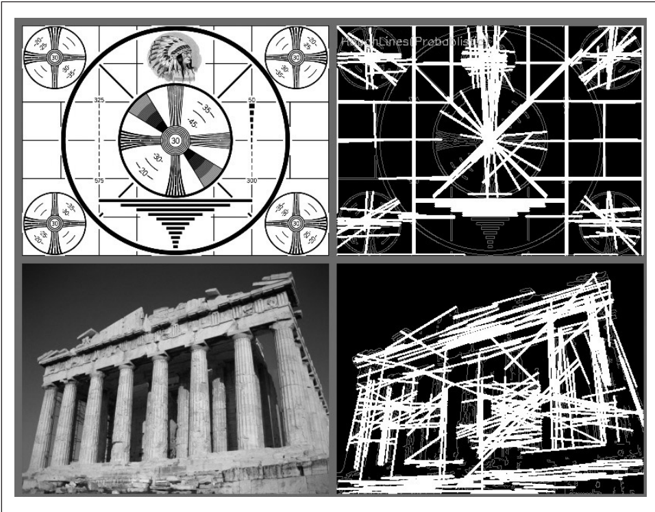
Figure 6-11. The Canny edge detector (param1=50, param2=150) is run first, with the results shown in gray, and the progressive probabilistic Hough transform (param1=50, param2=10) is run next, with the results overlaid in white; you can see that the strong lines are generally picked up by the Hough transform
