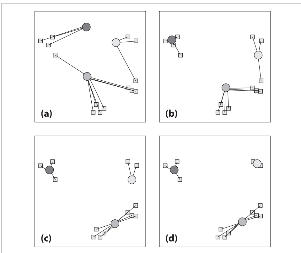
Figure 13-5. K-means in action for two iterations: (a) cluster centers are placed randomly and each data point is then assigned to its nearest cluster center; (b) cluster centers are moved to the centroid of their points; (c) data points are again assigned to their nearest cluster centers; (d) cluster centers are again moved to the centroid of their points
