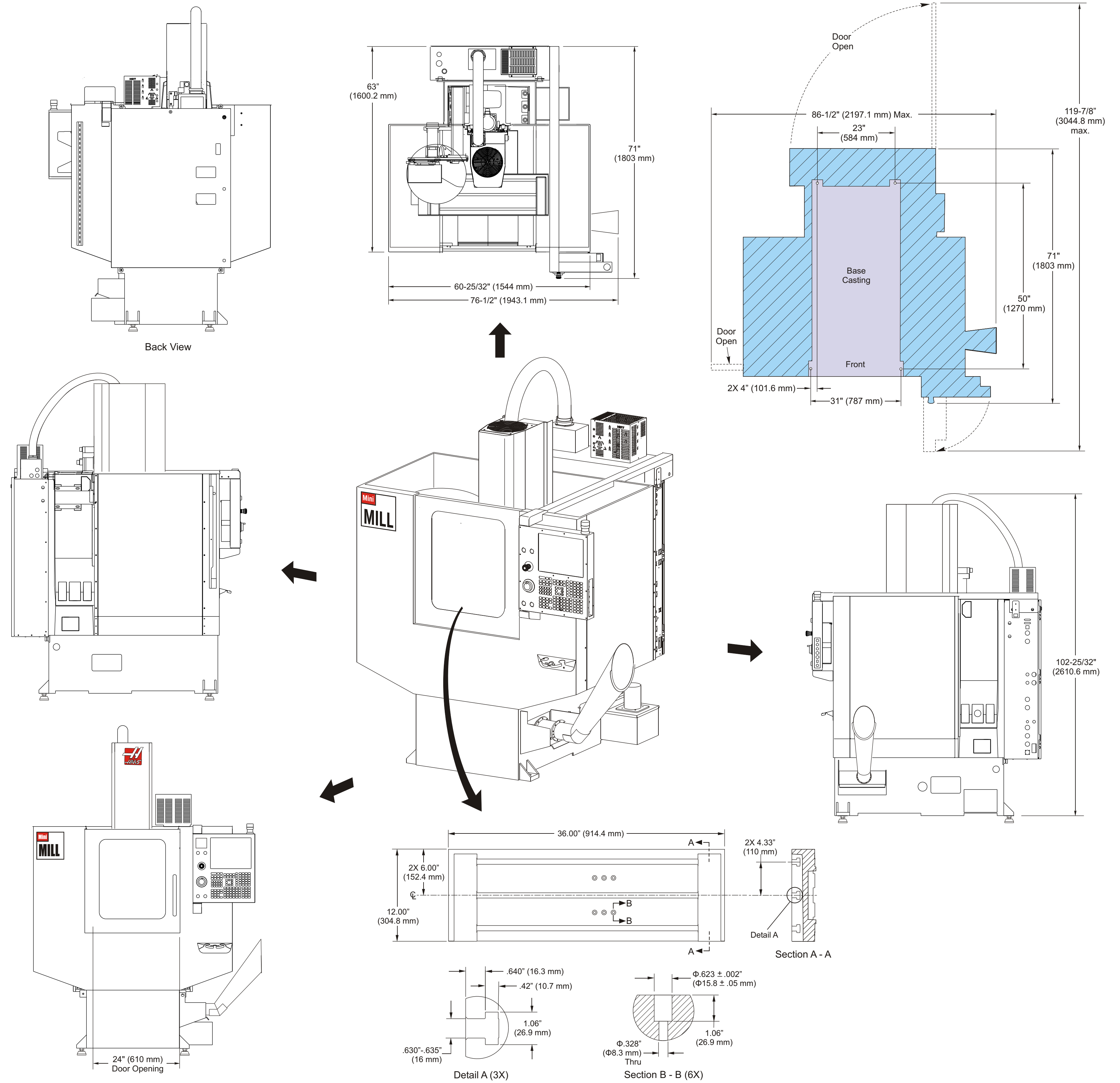
Mini-Mill Table Dimensions
