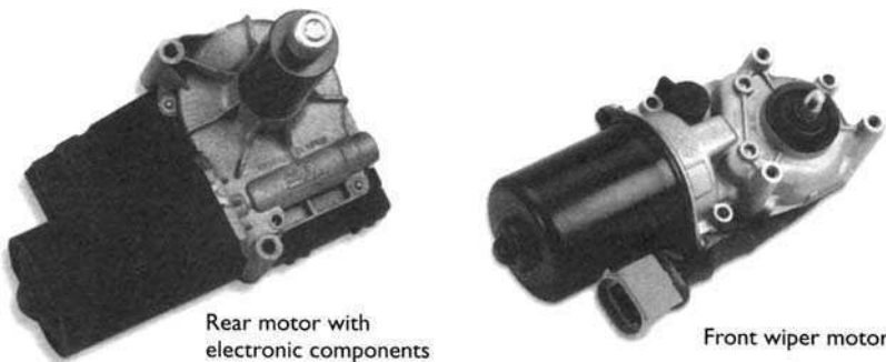
Figure 9.17 Wiper motors
