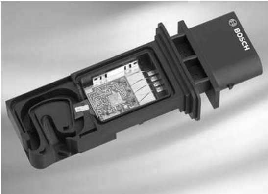
Figure 6.12 Hot film mass airflow sensor
