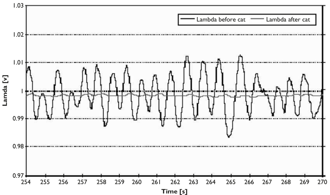
Figure 5.7 Upstream and downstream exhaust gas sensor activity – good catalyst (Source: SAE 2001-01-0933 New Cat Preparation Procedure for OBD2 Monitoring Requirements)
