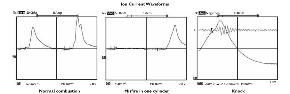
Figure 5.27 Resulting waveforms from the ion sensing system
