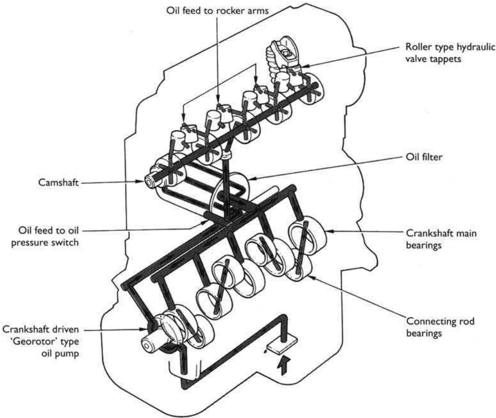
Figure 7.52 Lubrication system
