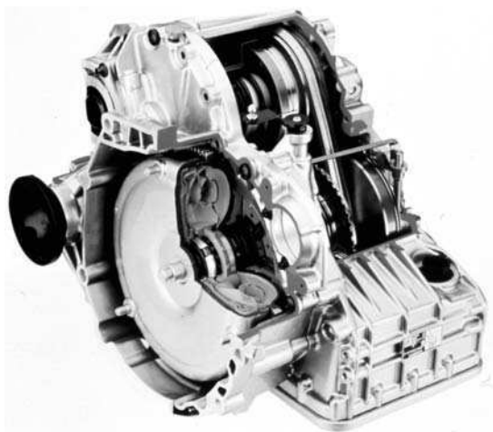
Figure 10.7 This cut-away gearbox shows the torque converter components
