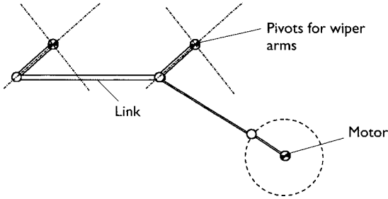
Figure 9.16 Wiper linkage
