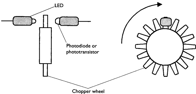
Figure 6.4 Optical sensor
