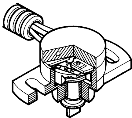
Figure 6.5 Throttle potentiometer
