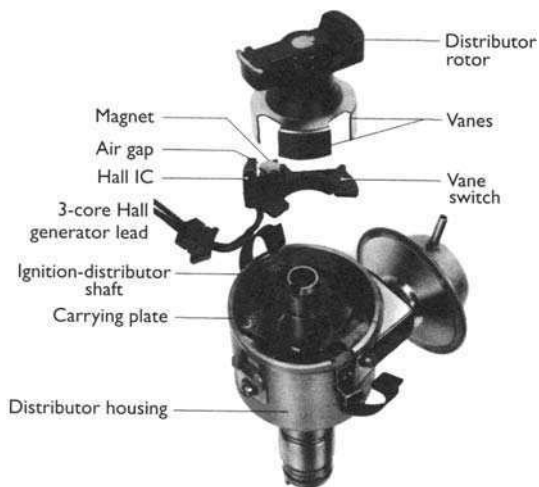
Figure 7.11 Ignition system with Hall generator
