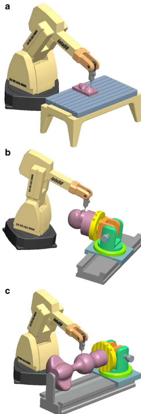
Fig. 1 a–c Conceptual model of reconfigurable robot-based multi-axis machining system
