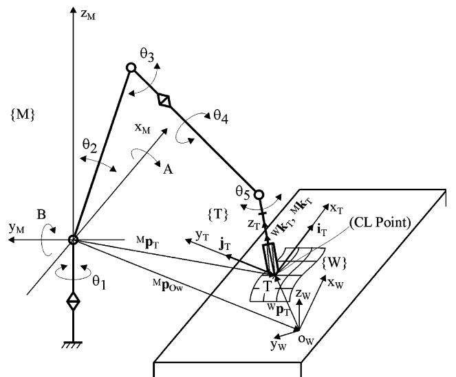
Fig. 3 Tool position and orientation in the work piece frame {W} and robot reference frame {M}
