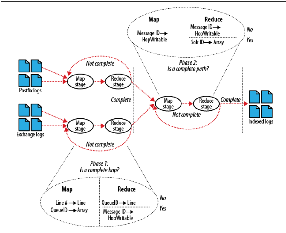
Figure 16-9. MapReduce chain
