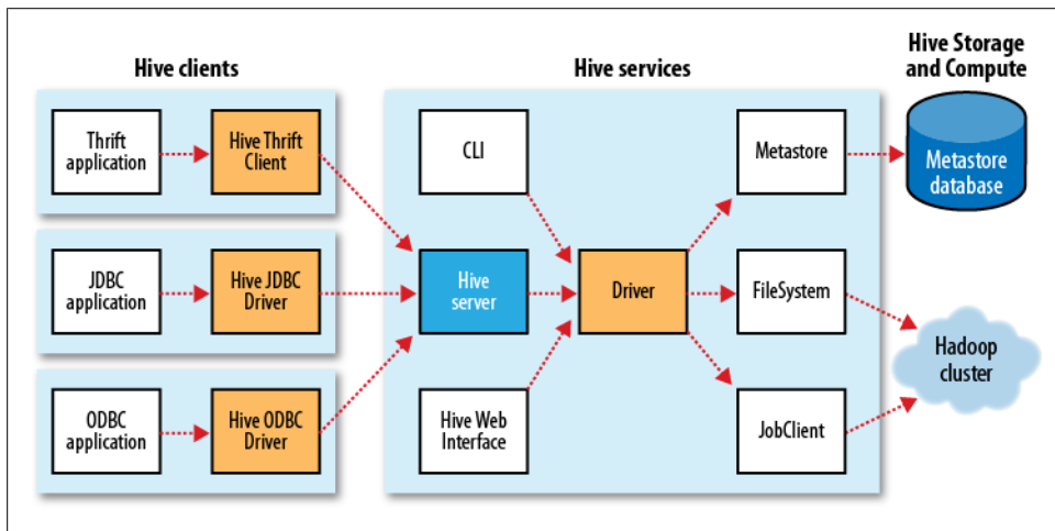
Figure 12-1. Hive architecture
