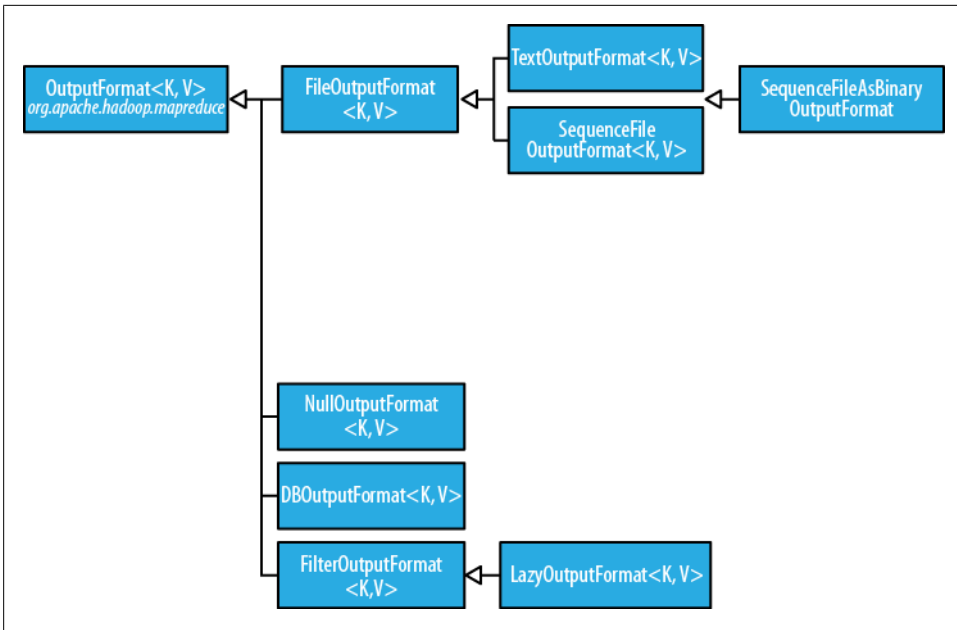
Figure 7-4. OutputFormat class hierarchy
