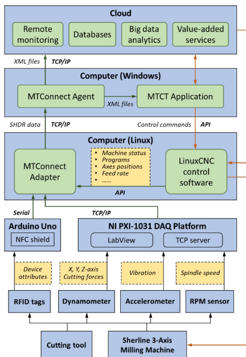
Fig. 3. Overall system architecture of MTConnect-based CPMT prototype
