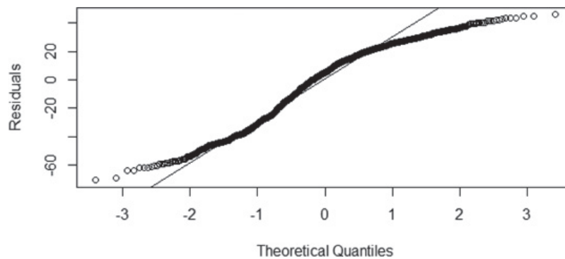
FIGURE 6-13 Q-Q plot of non-normally distributed residuals
