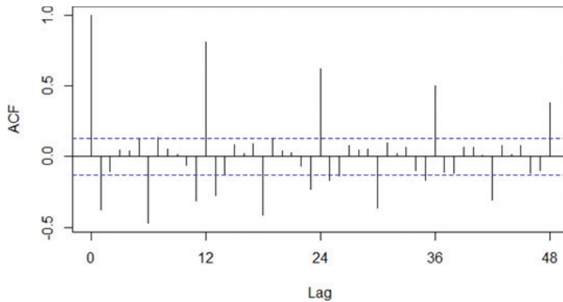
FIGURE 8-13 ACF of the differenced gasoline time series
