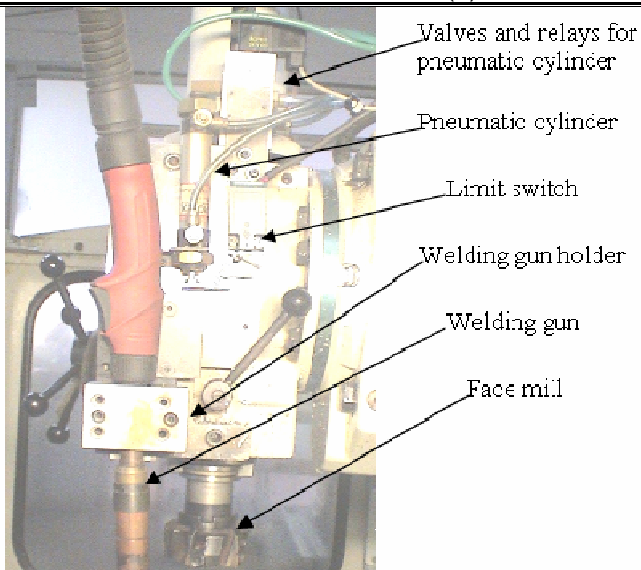
(b) Torch mounted on the spindle head
