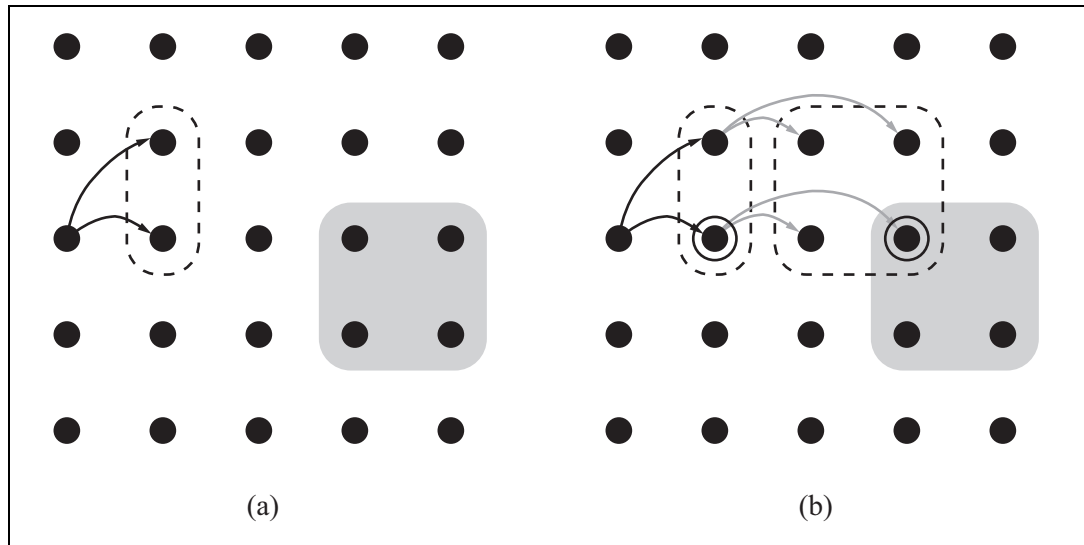
Figure 11.6 Schematic examples of reachable sets. The set of goal states is shaded. Black and gray arrows indicate possible implementations of h_1 and h_2 , respectively. (a) The reachable set of an HLA h_1 in a state s . (b) The reachable set for the sequence [h_1, h_2] . Because this intersects the goal set, the sequence achieves the goal.
