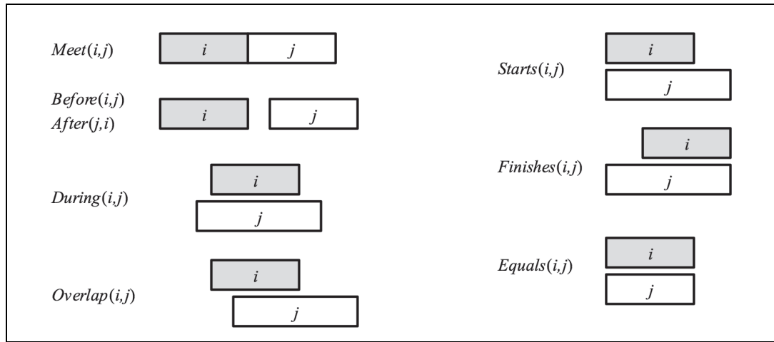
Figure 12.2 Predicates on time intervals.
