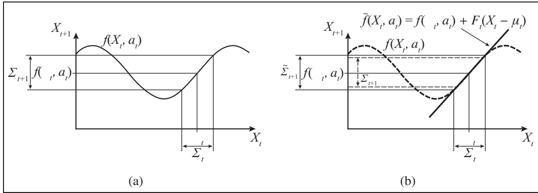
Figure 25.11 One-dimensional illustration of a linearized motion model: (a) The function f , and the projection of a mean \mu_t and a covariance interval (based on \Sigma_t ) into time t + 1 . (b) The linearized version is the tangent of f at \mu_t . The projection of the mean \mu_t is correct. However, the projected covariance \tilde{\Sigma}_{t+1} differs from \Sigma_{t+1} .
