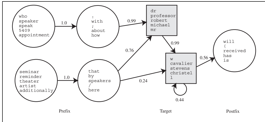
Figure 22.2 Hidden Markov model for the speaker of a talk announcement. The two square states are the target (note the second target state has a self-loop, so the target can match a string of any length), the four circles to the left are the prefix, and the one on the right is the postfix. For each state, only a few of the high-probability words are shown. From Freitag and McCallum (2000).
