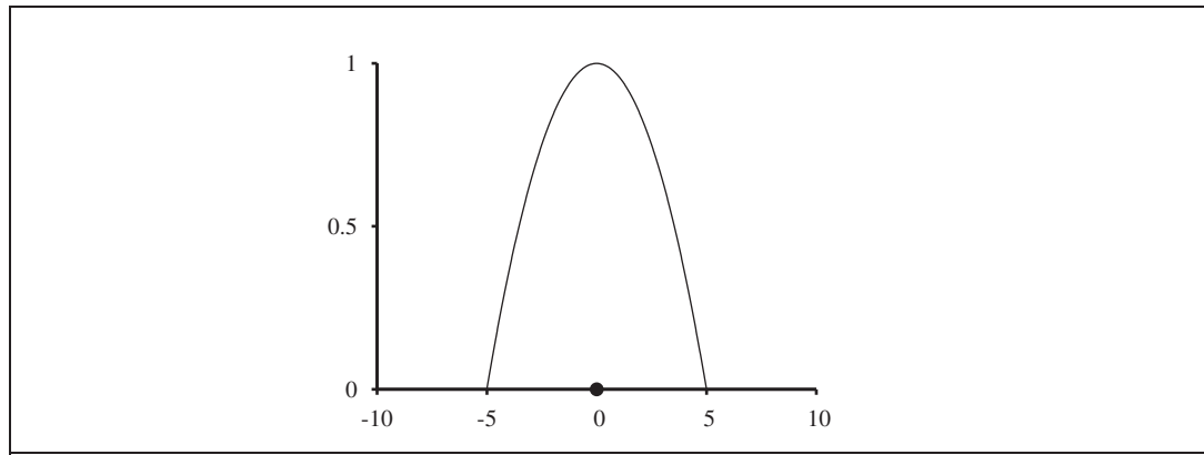
Figure 18.29 A quadratic kernel, \mathcal{K}(x) = \max(0, 1 - (2|x|)^2) , with kernel width = 10, centered on the query point = 0.
