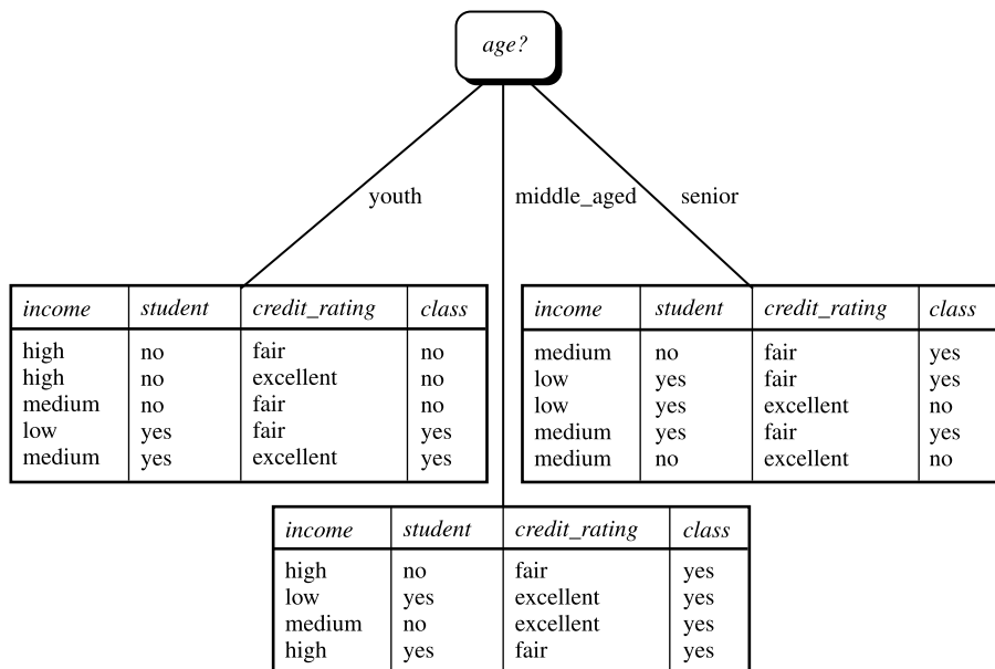
Figure 8.5 The attribute \text{age} has the highest information gain and therefore becomes the splitting attribute at the root node of the decision tree. Branches are grown for each outcome of \text{age} . The tuples are shown partitioned accordingly.
