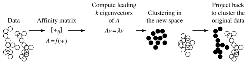
Figure 11.10 The framework of spectral clustering approaches. Source: Adapted from Slide 8 at http://videolectures.net/micued08_azran_mcl/ .
