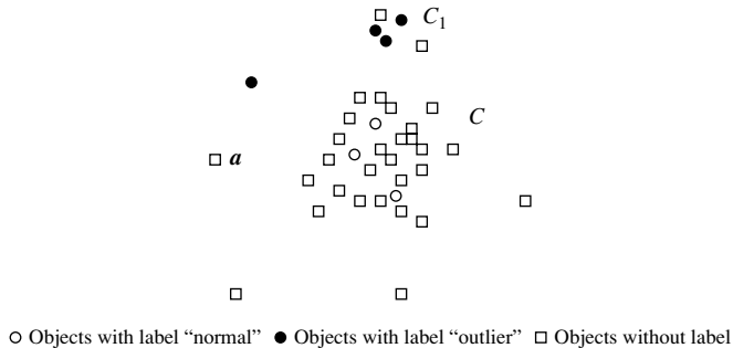
Figure 12.14 Detecting outliers by semi-supervised learning.
